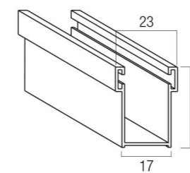
Guida in alluminio A28 GUAL..28M 17 x 28 mm
